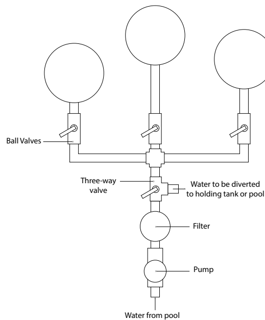
Spheres at Different Distances Use individual flow control valves
