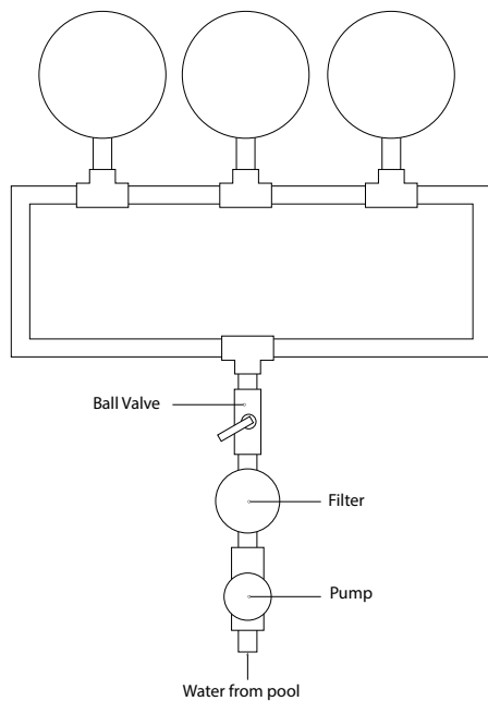
Spheres at equal distances Use looped plumbing
